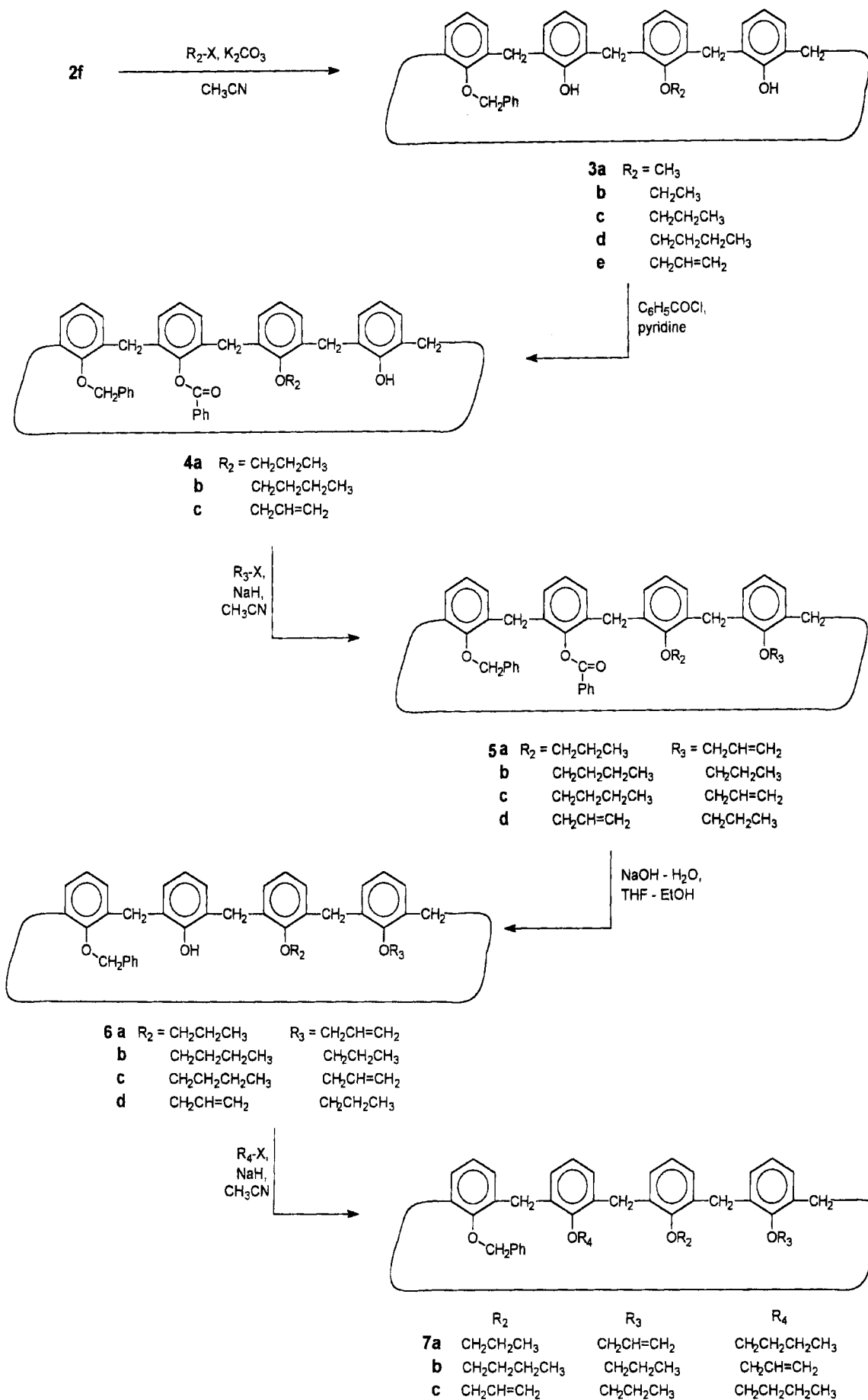
Figure 2. Synthesis of calix[4]arenes with four different "lower rim" substituents.
