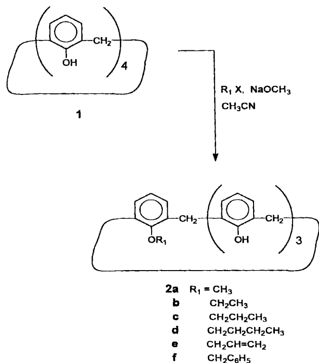
Figure 1. Monoalkoxycalix[4]arenes.
